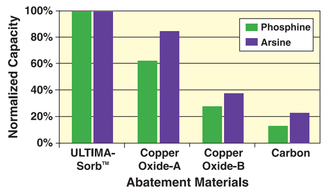
Figure 1: ULTIMA-Sorb™ delivers much higher capacity for PH_3 and AsH_3 than conventional copper oxide-based abatement material and activated carbon-based material.
