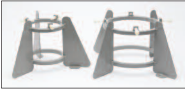
Figure 5 – Model 700 and 701 Small Cylinder Stands
