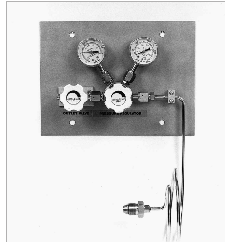
Model 9001 ULTRA-LINE® Pressure Control Module shown with regulator and outlet valve (regulator and outlet valve sold separately).
