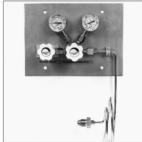
Model 9001 ULTRA-LINE® Pressure Control Module shown with regulator and outlet valve (regulator and outlet valve sold separately).
