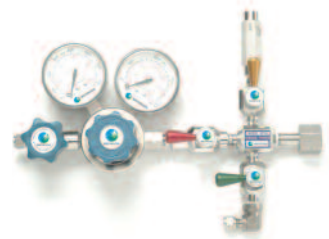
Model 4774 Cross Purge Assembly, shown with a Model 3210 Deluxe Corrosive Service Regulator
